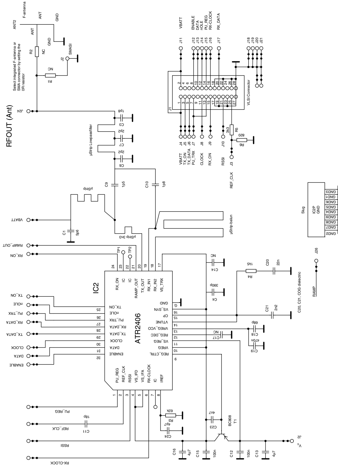
Figure 7. Application Circuit
